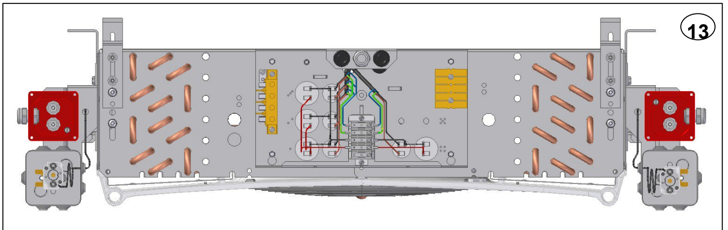
RACCORDEMENT ELECTRIQUE - ELECTRICAL WIRING ELEKTRISCHE ANSCHLÜSSE - CONEXIONES ELECTRICAS
